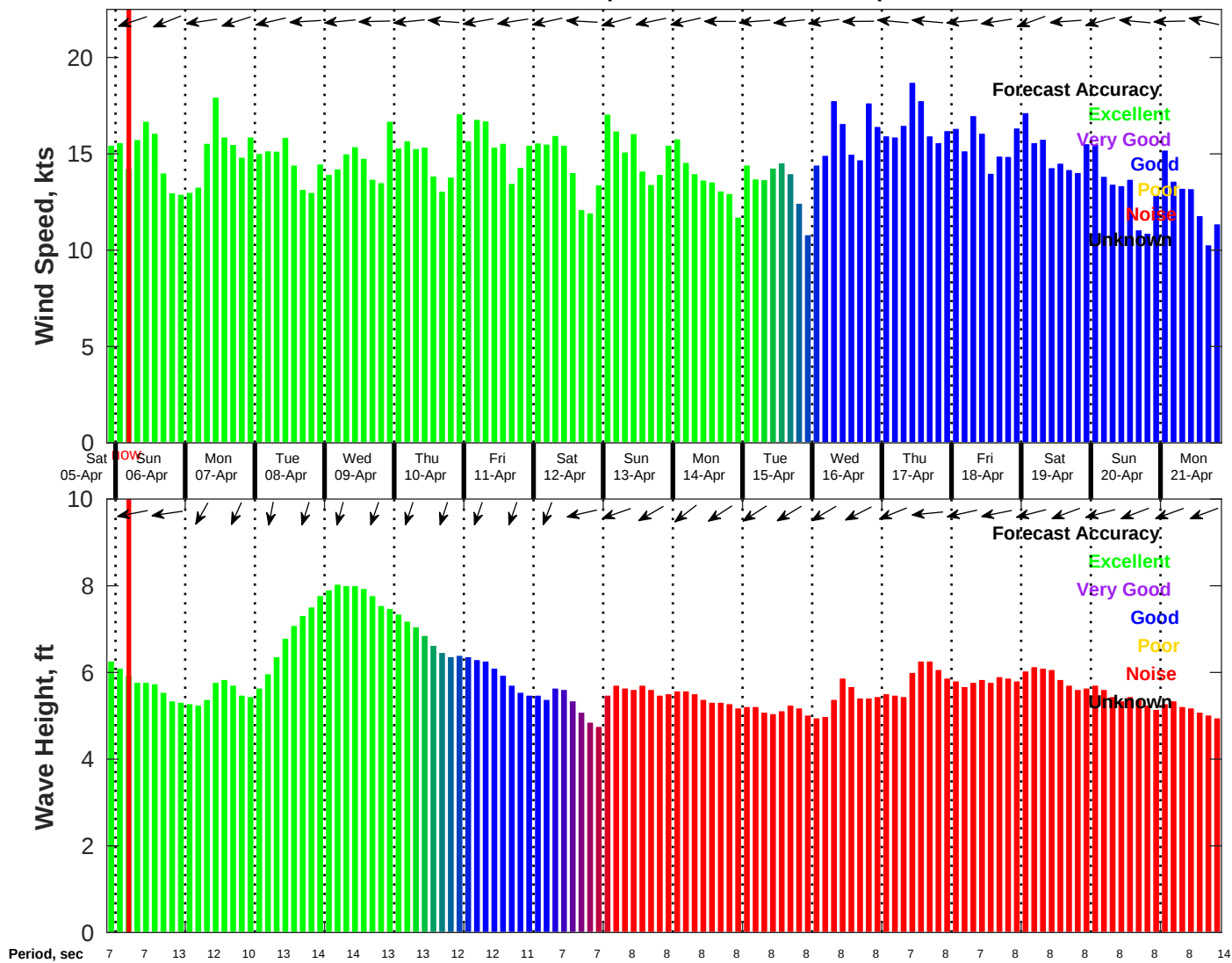
Wind & Wave Forecast for NDBC 41040 from 05-Apr-2025 21:00:00 to 21-Apr-2025 21:00:00
