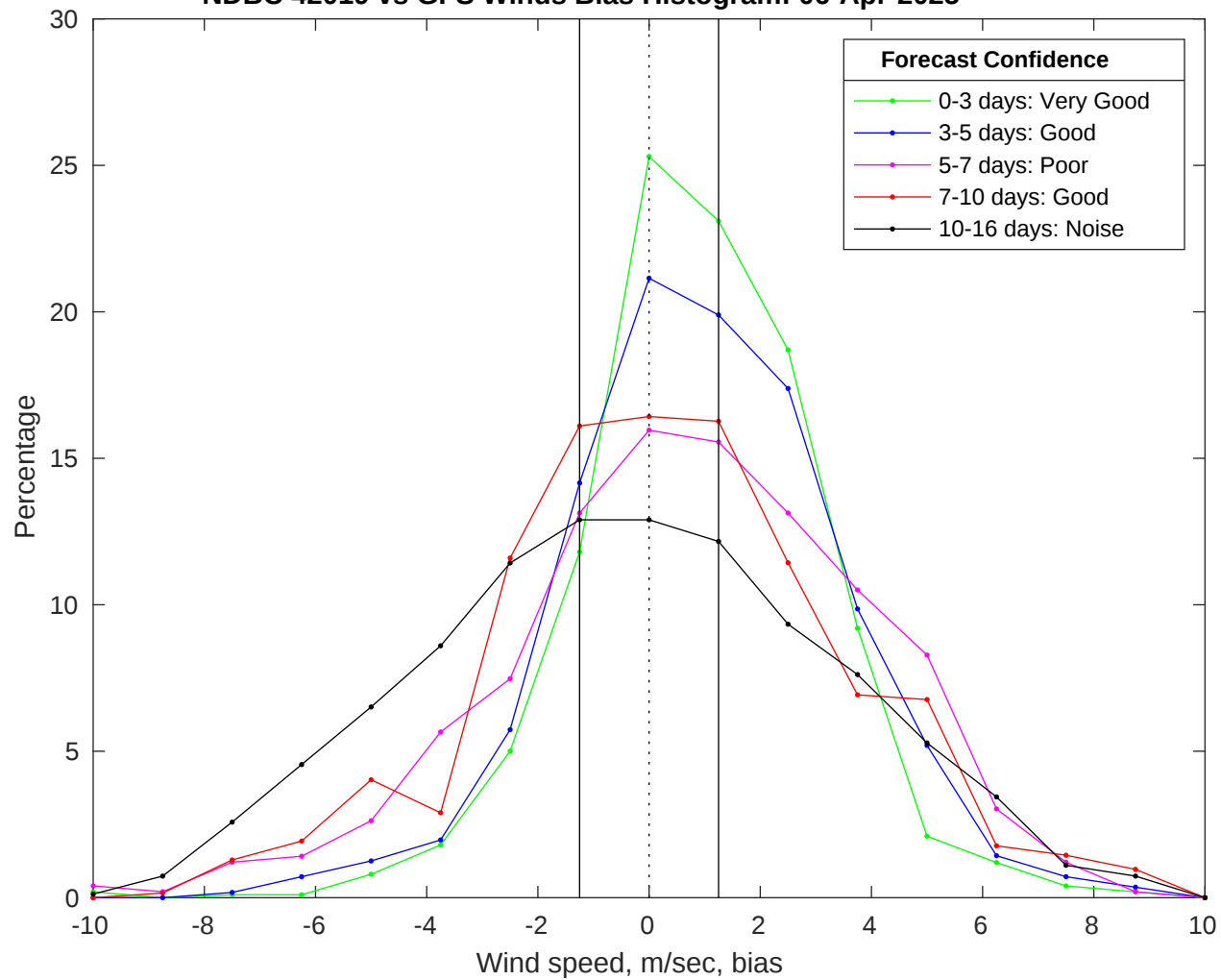
NDBC 42019 vs GFS Winds Bias Histogram: 06-Apr-2025
