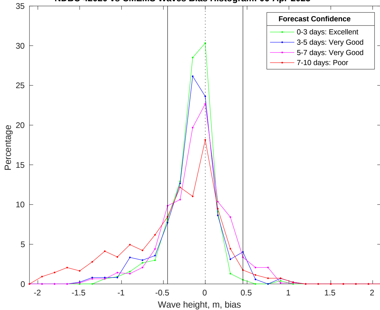
NDBC 42020 vs CMEMS Waves Bias Histogram: 06-Apr-2025
