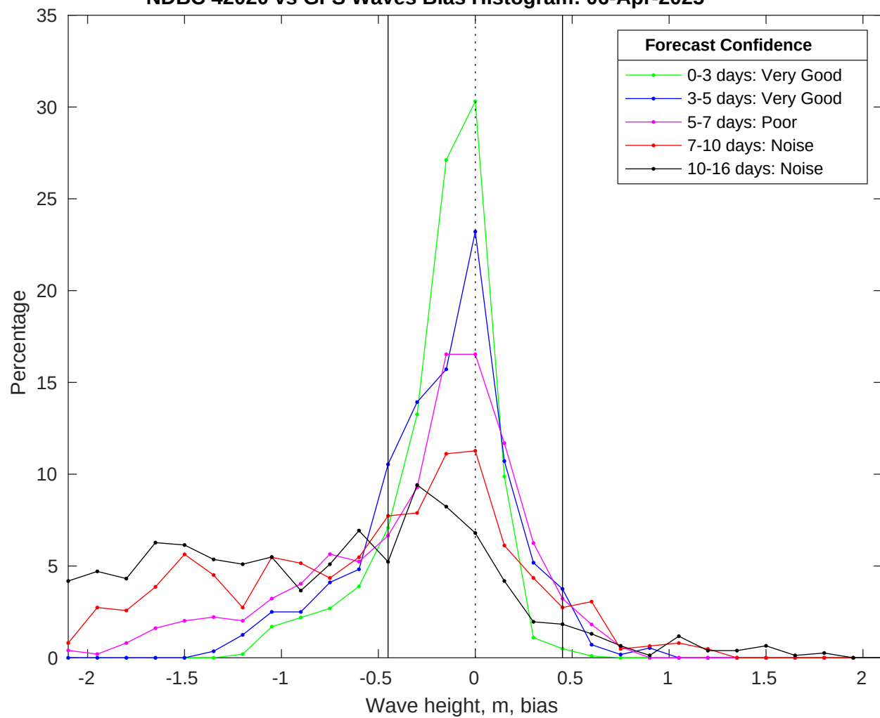
NDBC 42020 vs GFS Waves Bias Histogram: 06-Apr-2025
