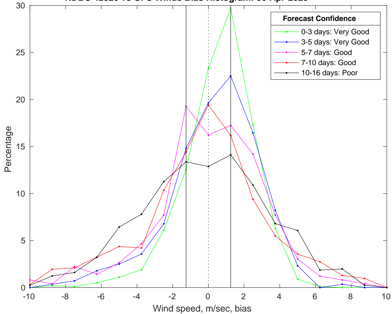
NDBC 42020 vs GFS Winds Bias Histogram: 06-Apr-2025
