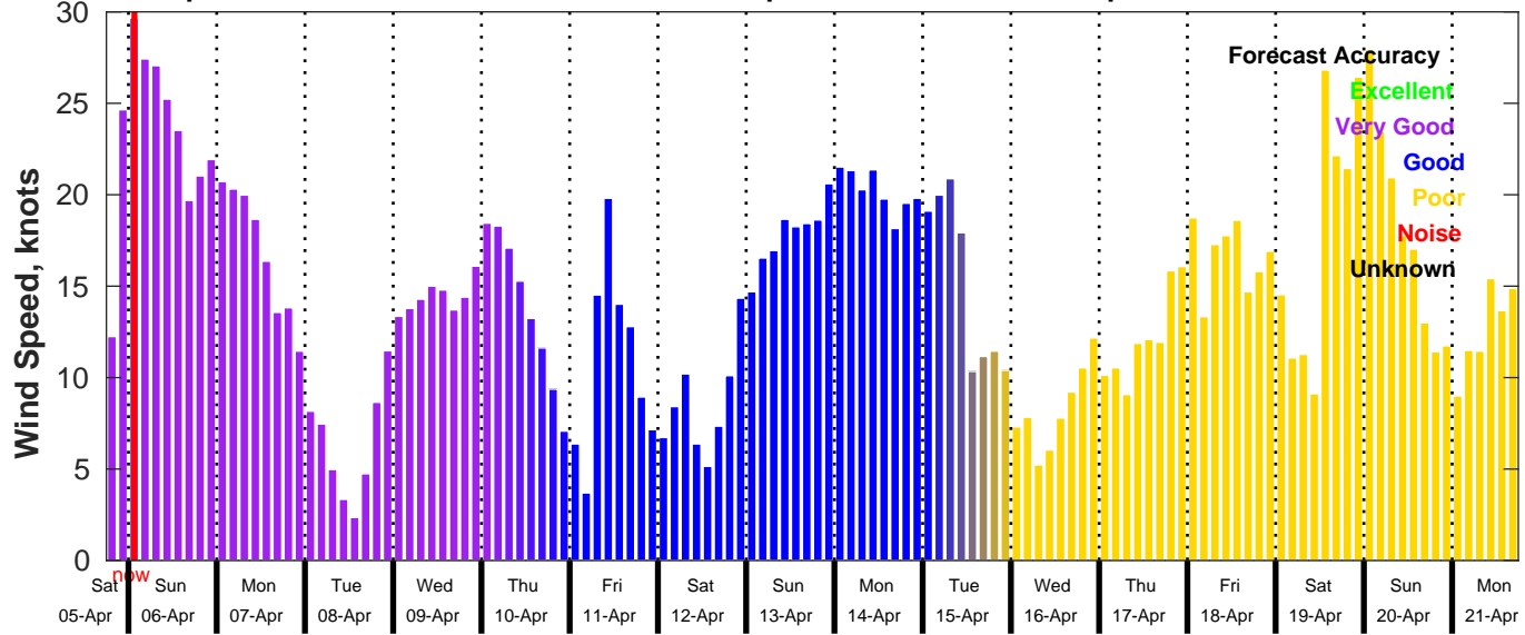
GFS Wind Speed Forecast for NDBC 42020 from 05-Apr-2025 18:00:00 to 21-Apr-2025 18:00:00
