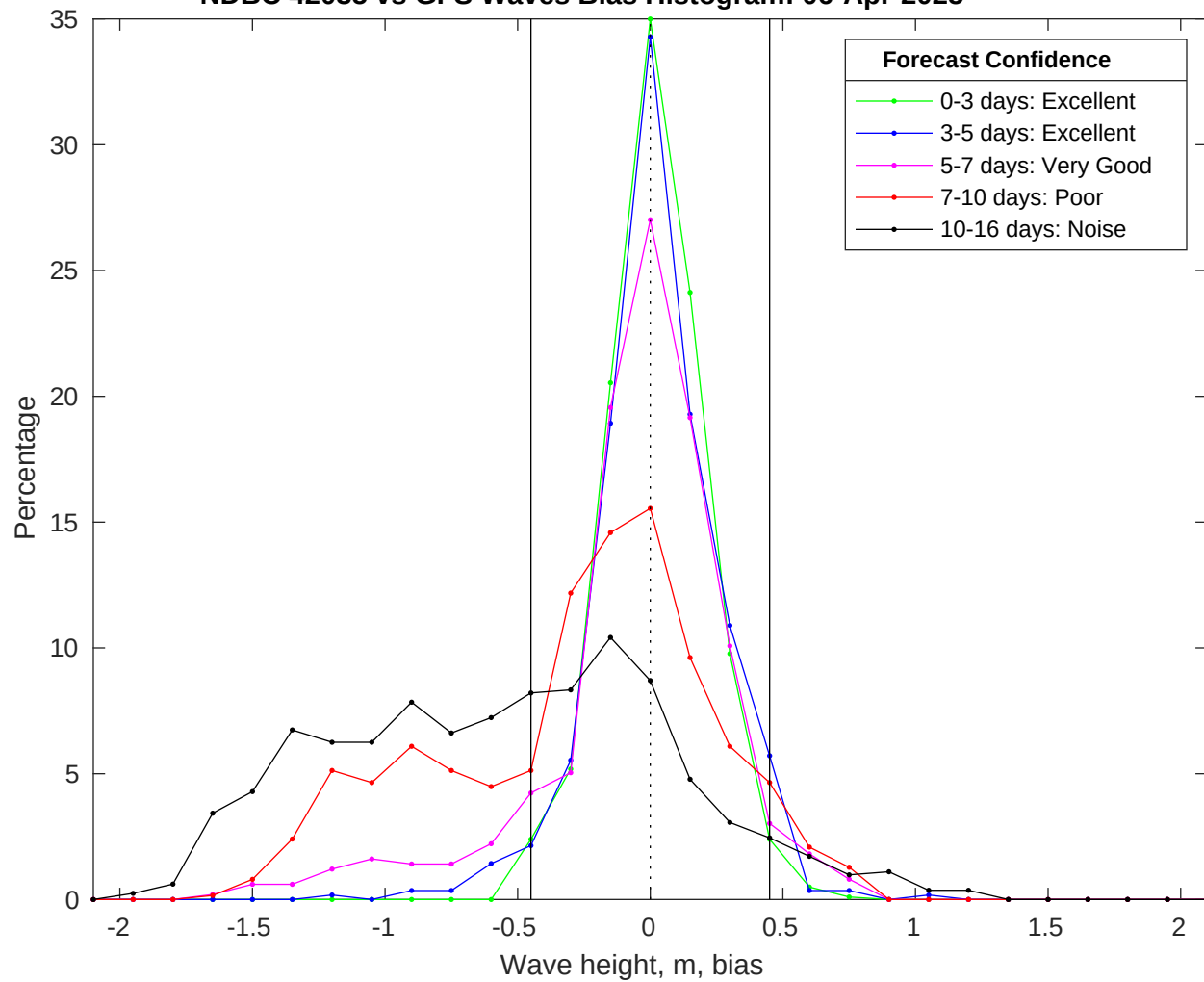
NDBC 42035 vs GFS Waves Bias Histogram: 06-Apr-2025
