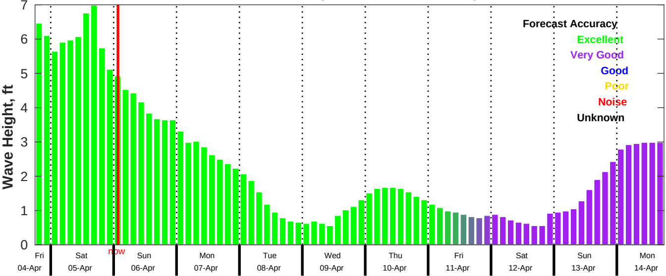
CMEMS Wave Forecast for NDBC 42035 from 04-Apr-2025 18:00:00 to 14-Apr-2025 18:00:00
