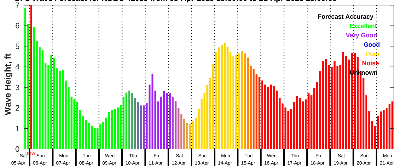
GFS Wave Forecast for NDBC 42035 from 05-Apr-2025 18:00:00 to 21-Apr-2025 18:00:00
