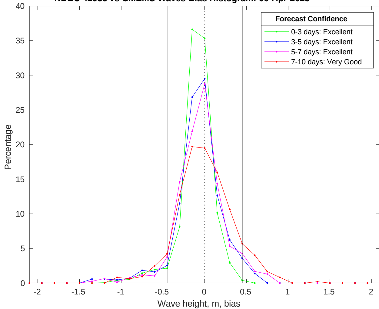
NDBC 42036 vs CMEMS Waves Bias Histogram: 06-Apr-2025
