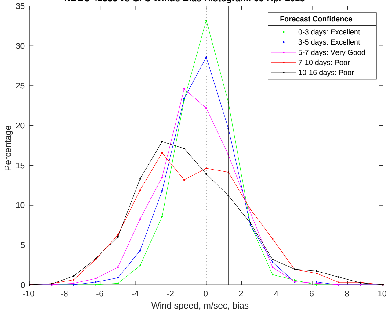
NDBC 42036 vs GFS Winds Bias Histogram: 06-Apr-2025
