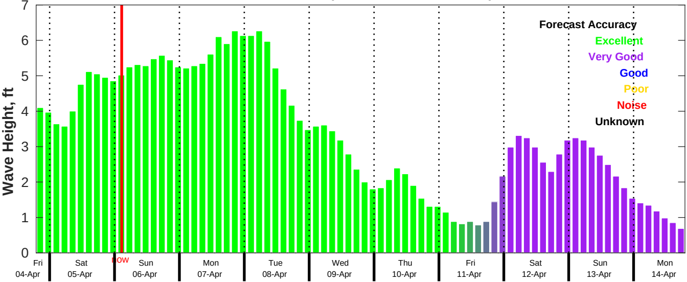
CMEMS Wave Forecast for NDBC 42036 from 04-Apr-2025 19:00:00 to 14-Apr-2025 19:00:00
