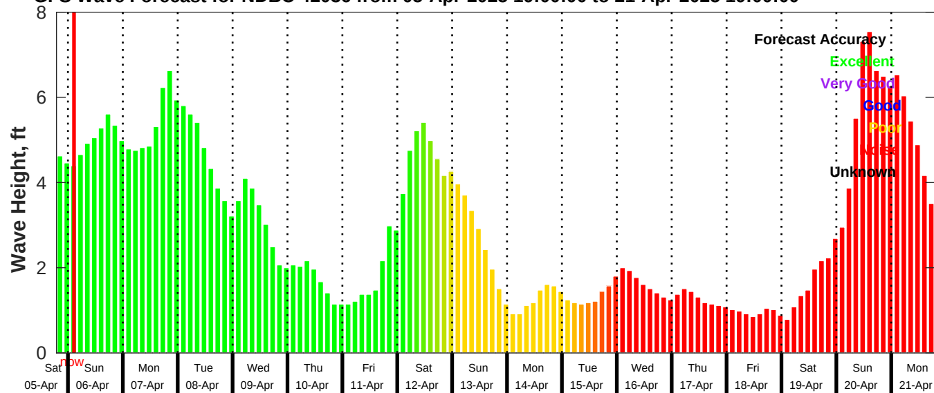
GFS Wave Forecast for NDBC 42036 from 05-Apr-2025 19:00:00 to 21-Apr-2025 19:00:00
