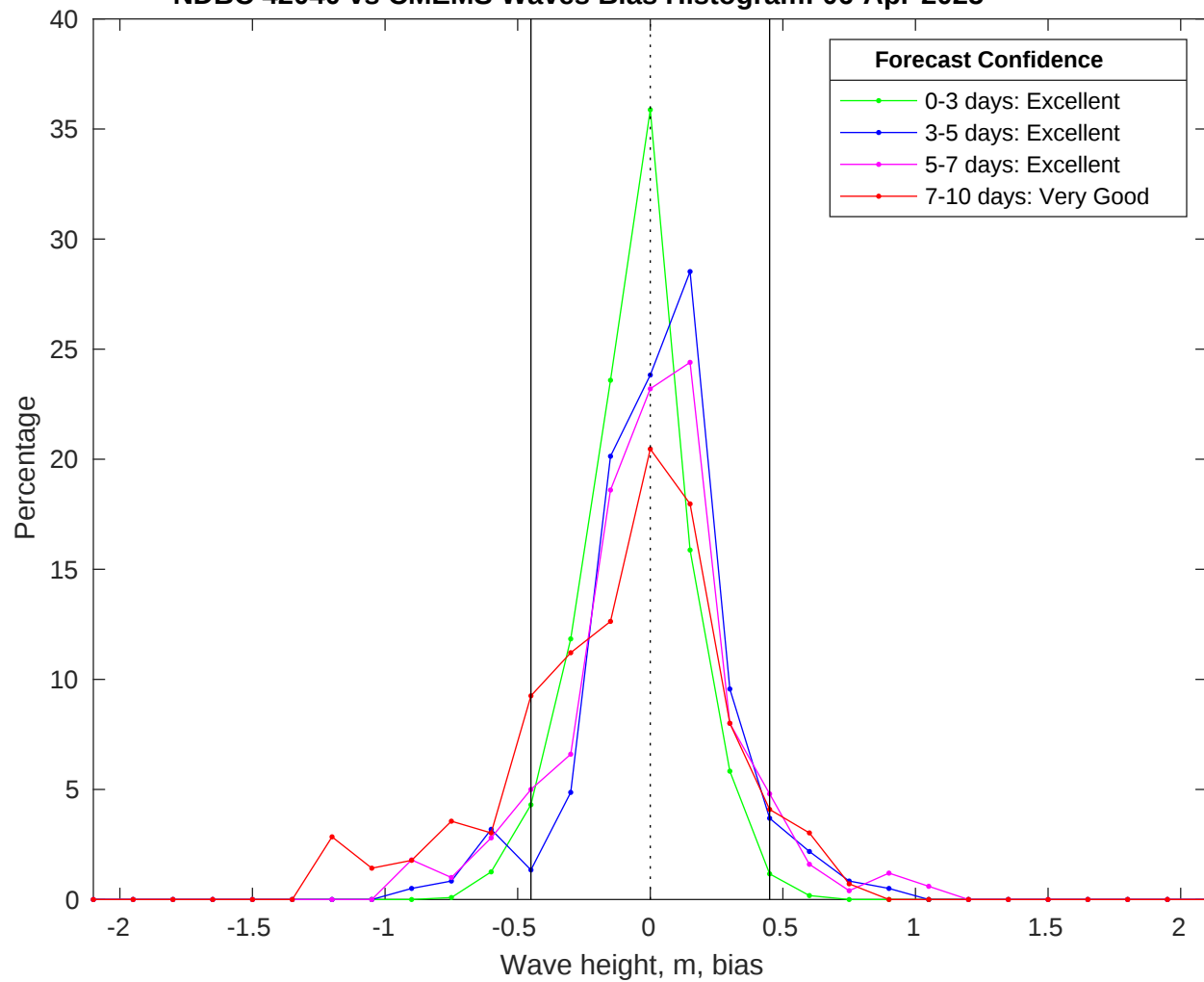
NDBC 42040 vs CMEMS Waves Bias Histogram: 06-Apr-2025
