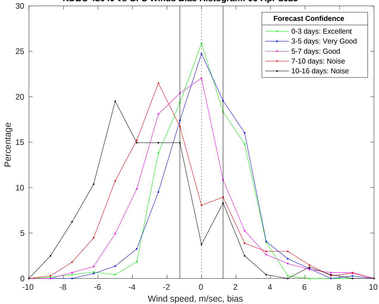
NDBC 42040 vs GFS Winds Bias Histogram: 06-Apr-2025
