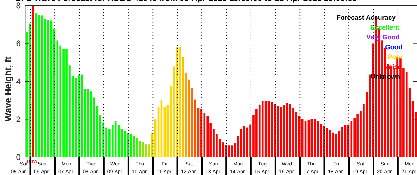
GFS Wave Forecast for NDBC 42040 from 05-Apr-2025 19:00:00 to 21-Apr-2025 19:00:00
