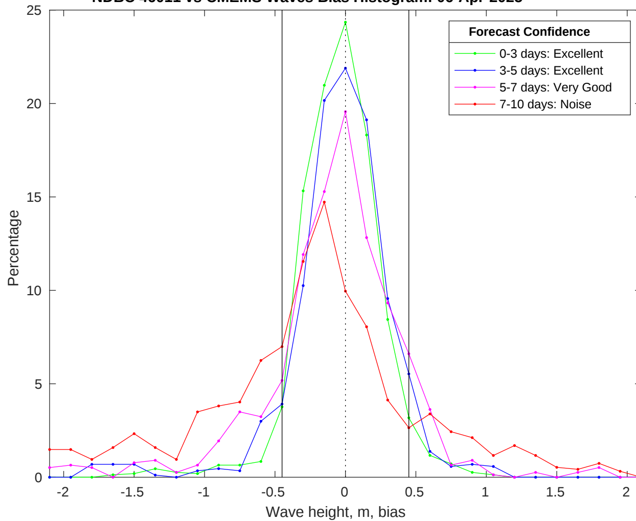
NDBC 46011 vs CMEMS Waves Bias Histogram: 06-Apr-2025
