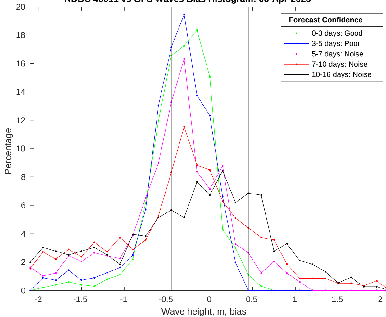
NDBC 46011 vs GFS Waves Bias Histogram: 06-Apr-2025
