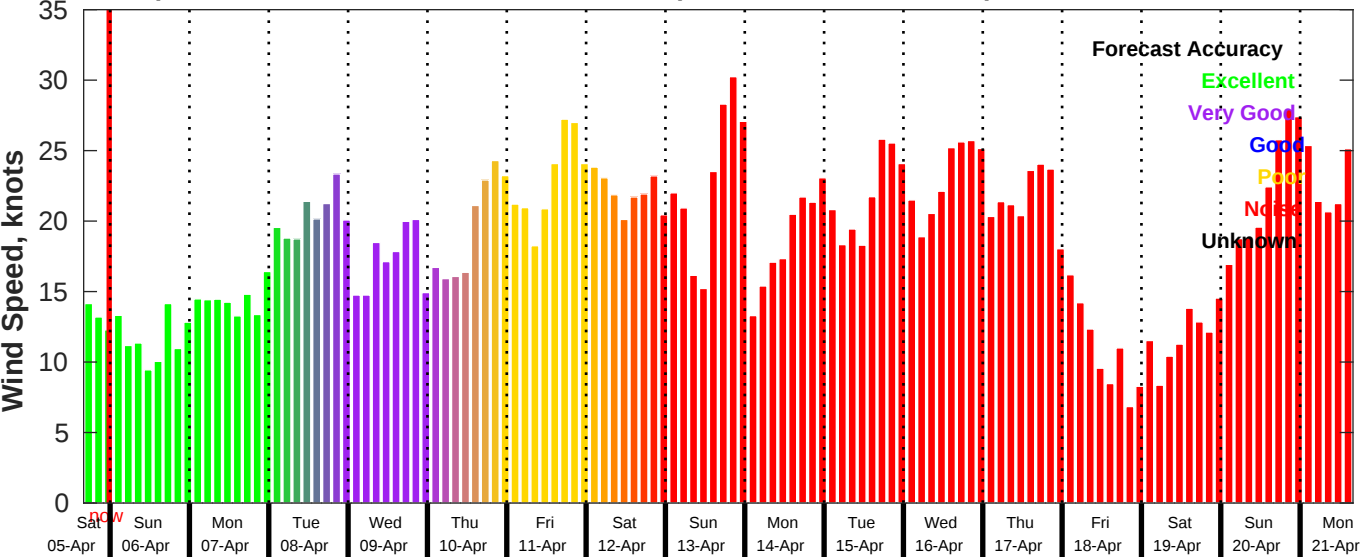
GFS Wind Speed Forecast for NDBC 46011 from 05-Apr-2025 16:00:00 to 21-Apr-2025 16:00:00
