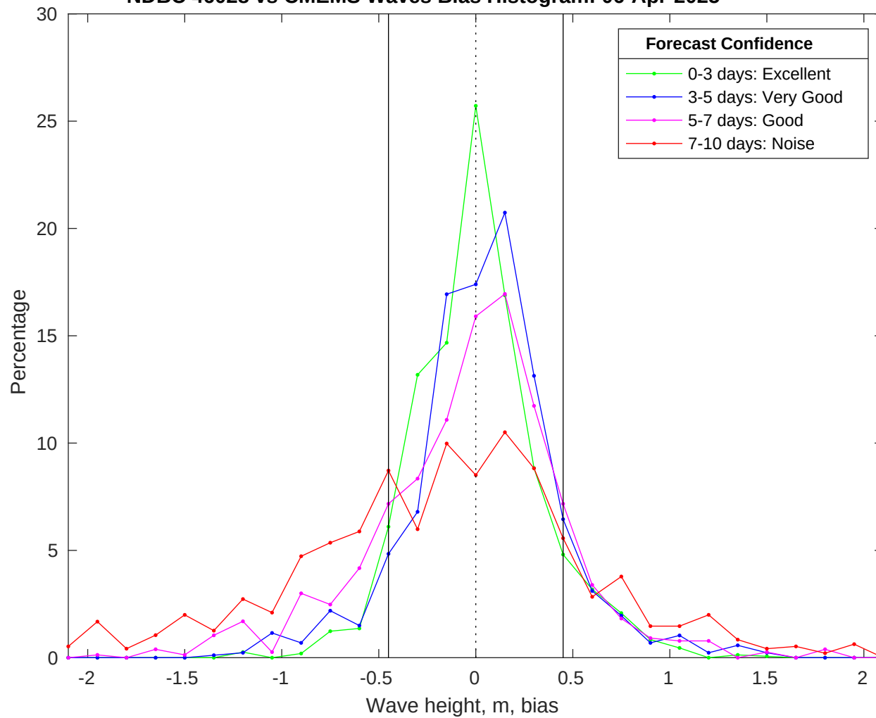
NDBC 46028 vs CMEMS Waves Bias Histogram: 06-Apr-2025
