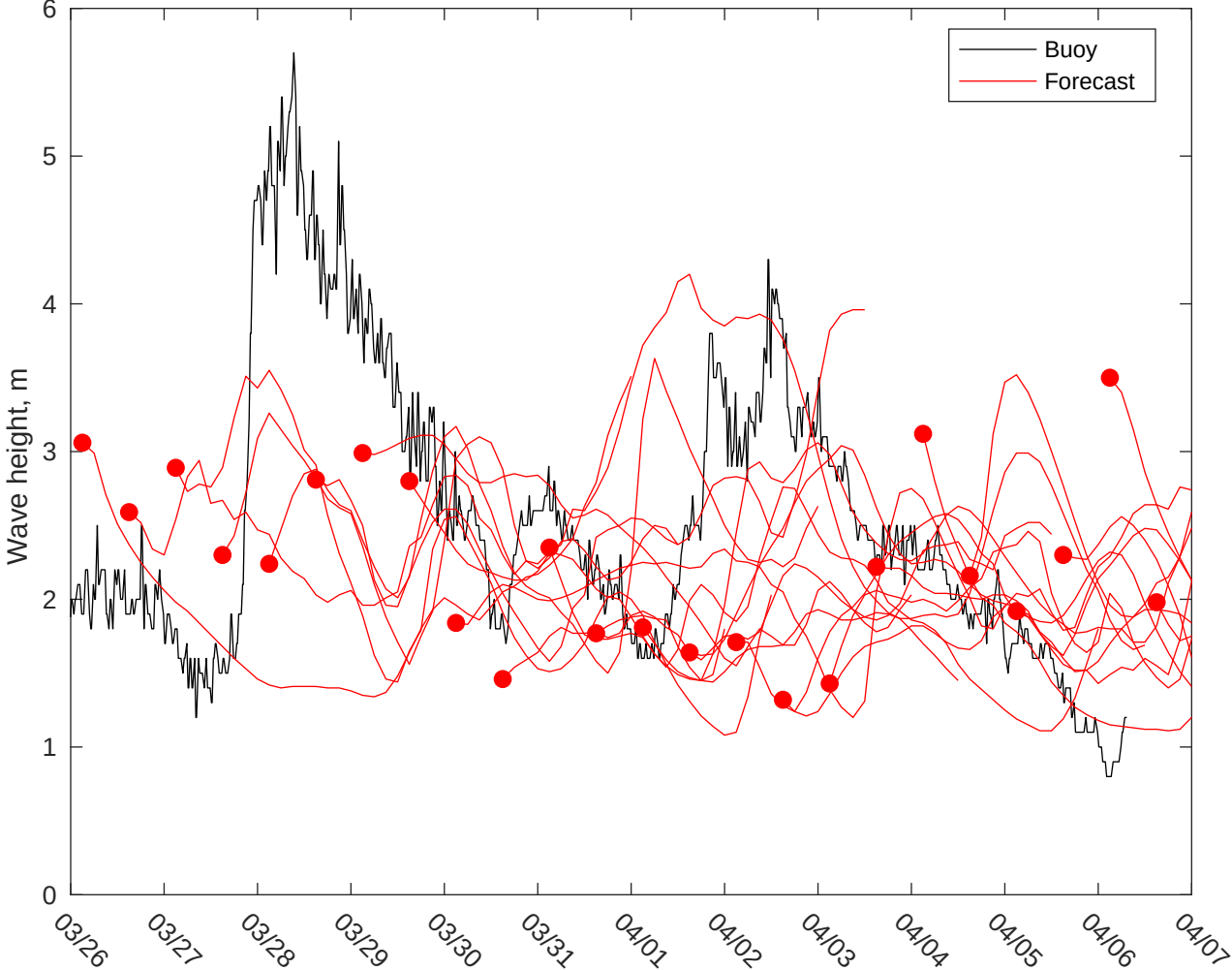
NDBC 46028 vs GFS Waves: 10 to 16 day forecast
