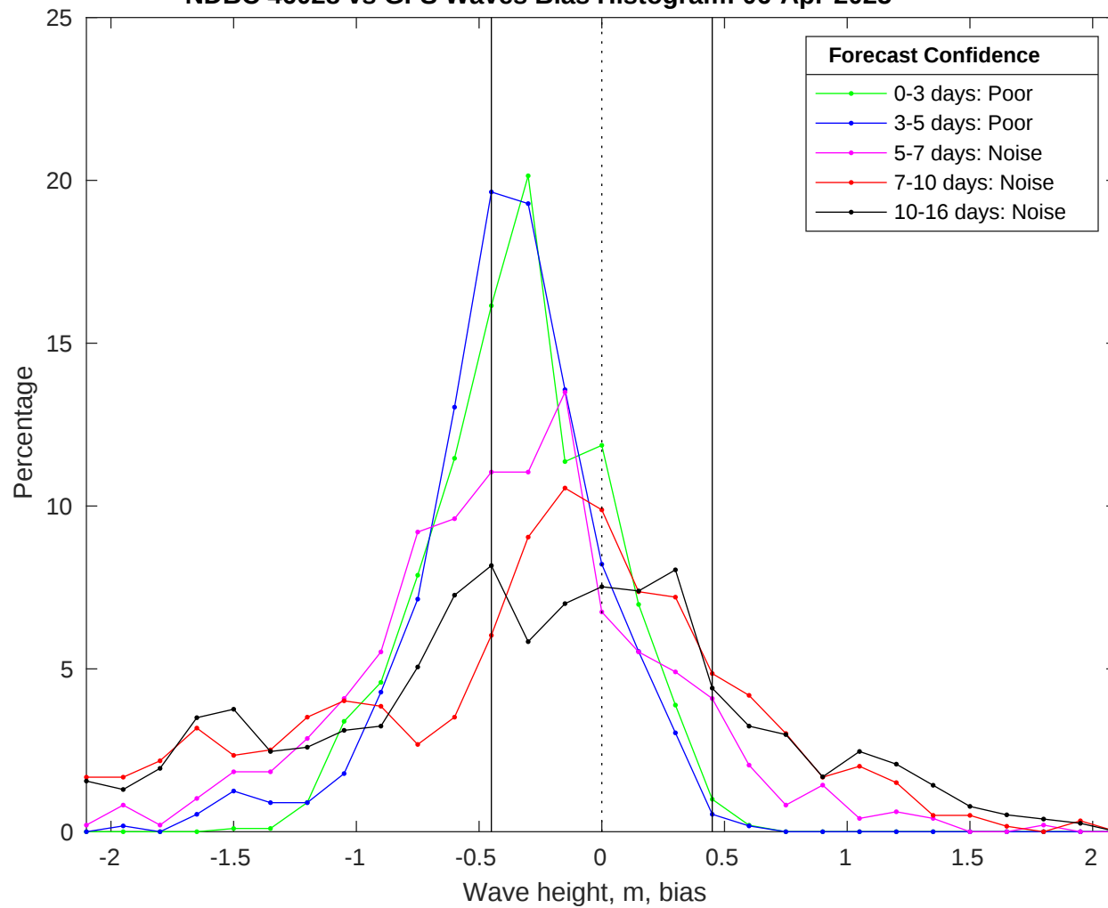
NDBC 46028 vs GFS Waves Bias Histogram: 06-Apr-2025
