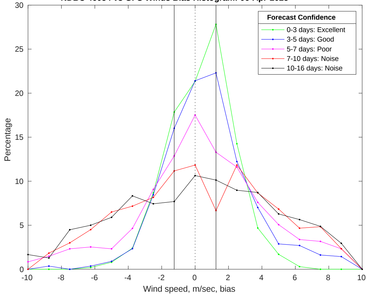
NDBC 46054 vs GFS Winds Bias Histogram: 06-Apr-2025
