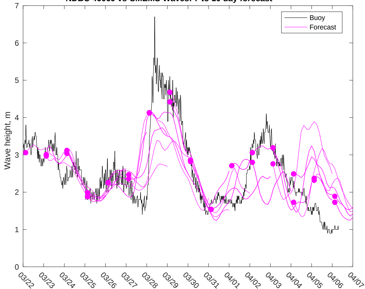
NDBC 46069 vs CMEMS Waves: 7 to 10 day forecast
