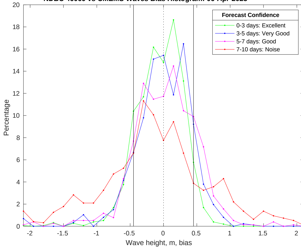
NDBC 46069 vs CMEMS Waves Bias Histogram: 06-Apr-2025
