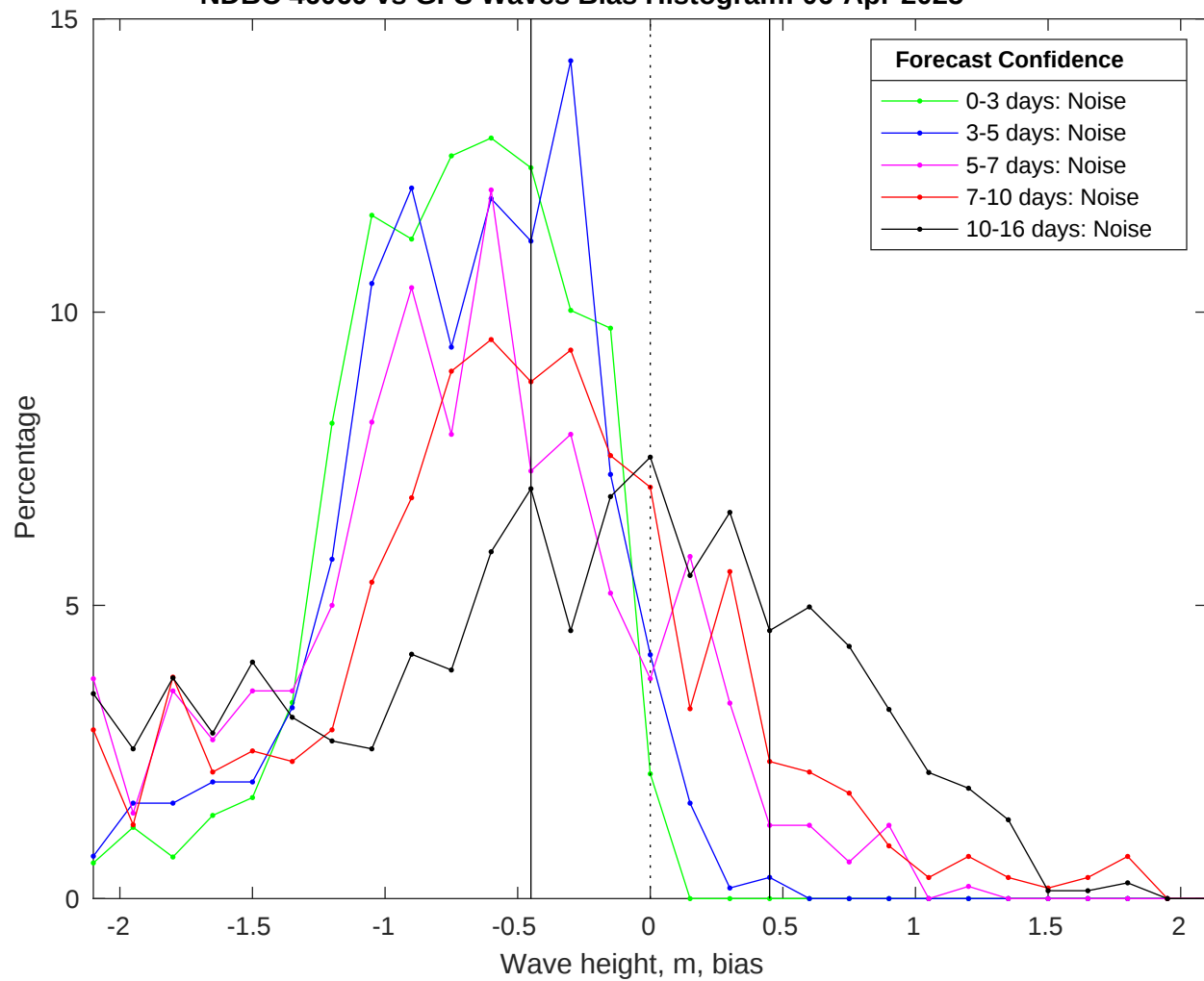
NDBC 46069 vs GFS Waves Bias Histogram: 06-Apr-2025
