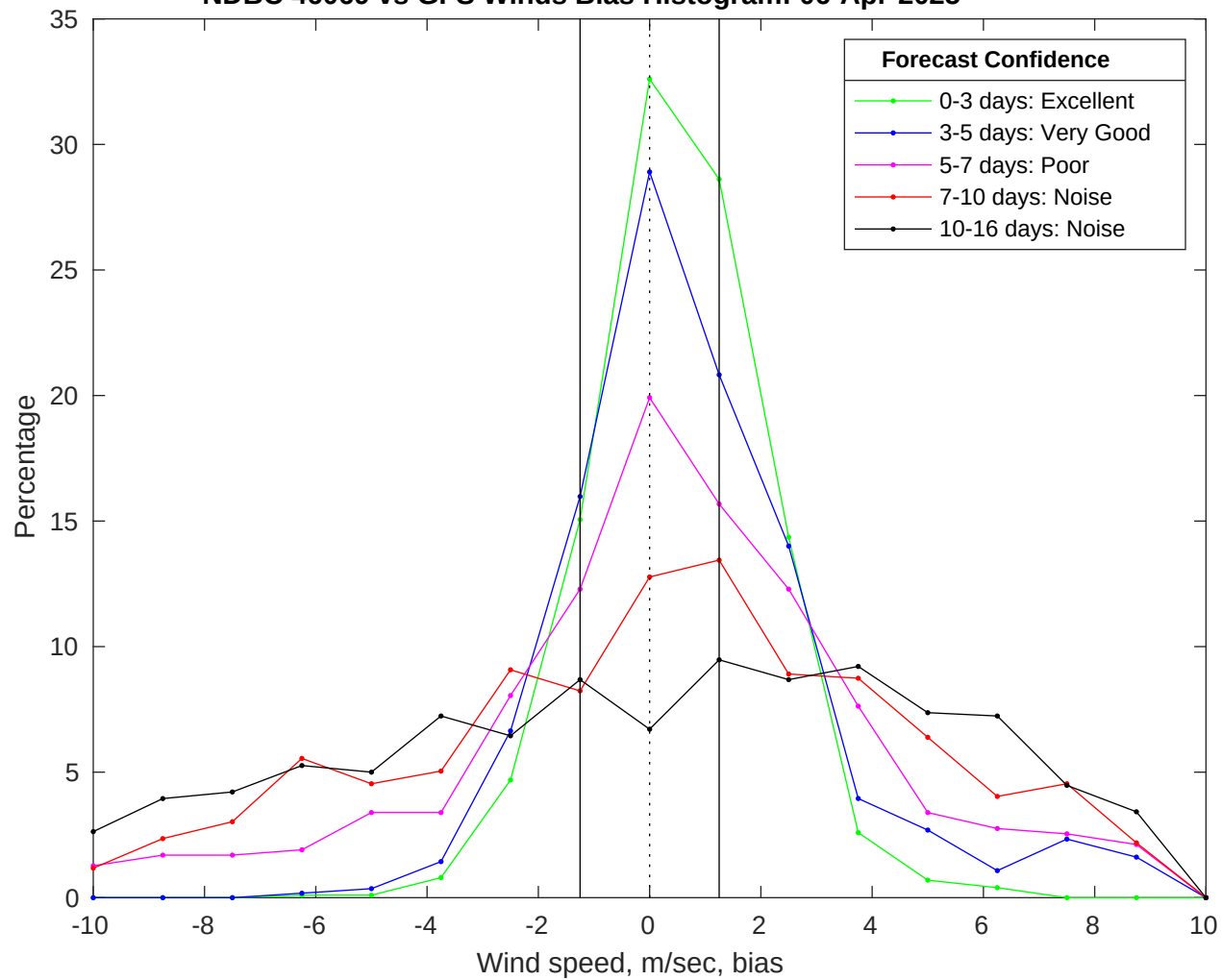
NDBC 46069 vs GFS Winds Bias Histogram: 06-Apr-2025
