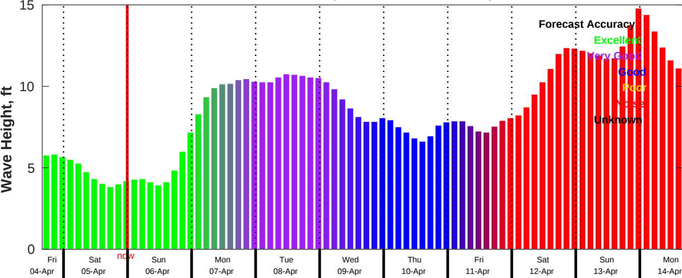
CMEMS Wave Forecast for NDBC 46069 from 04-Apr-2025 16:00:00 to 14-Apr-2025 16:00:00
