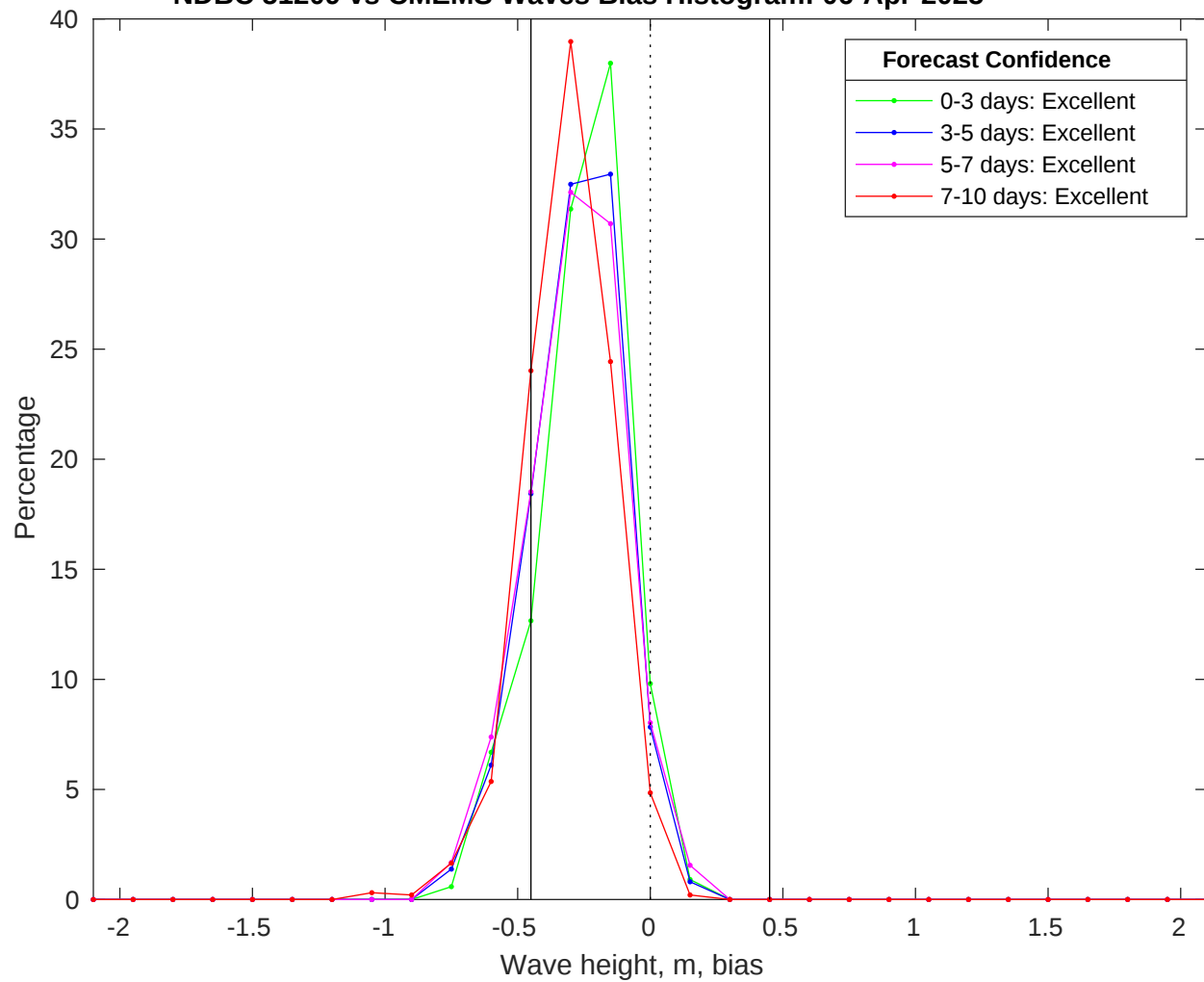
NDBC 51209 vs CMEMS Waves Bias Histogram: 06-Apr-2025
