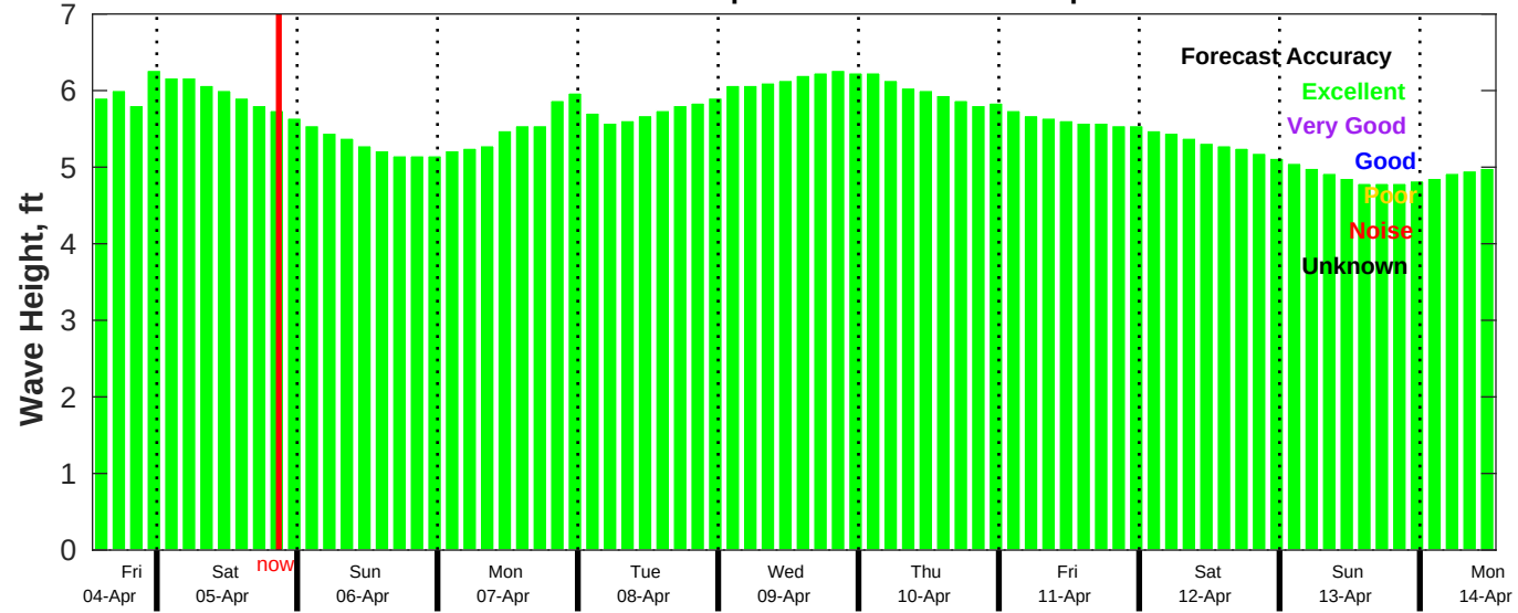
CMEMS Wave Forecast for NDBC 51209 from 04-Apr-2025 13:00:00 to 14-Apr-2025 13:00:00
