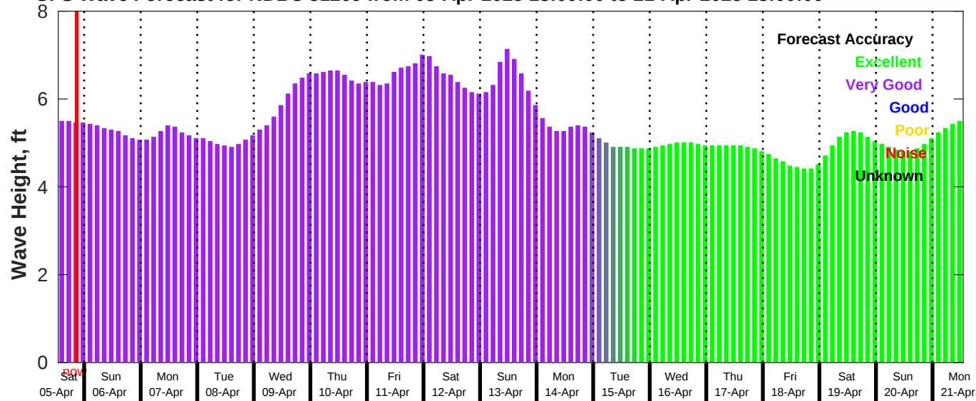
GFS Wave Forecast for NDBC 51209 from 05-Apr-2025 13:00:00 to 21-Apr-2025 13:00:00
