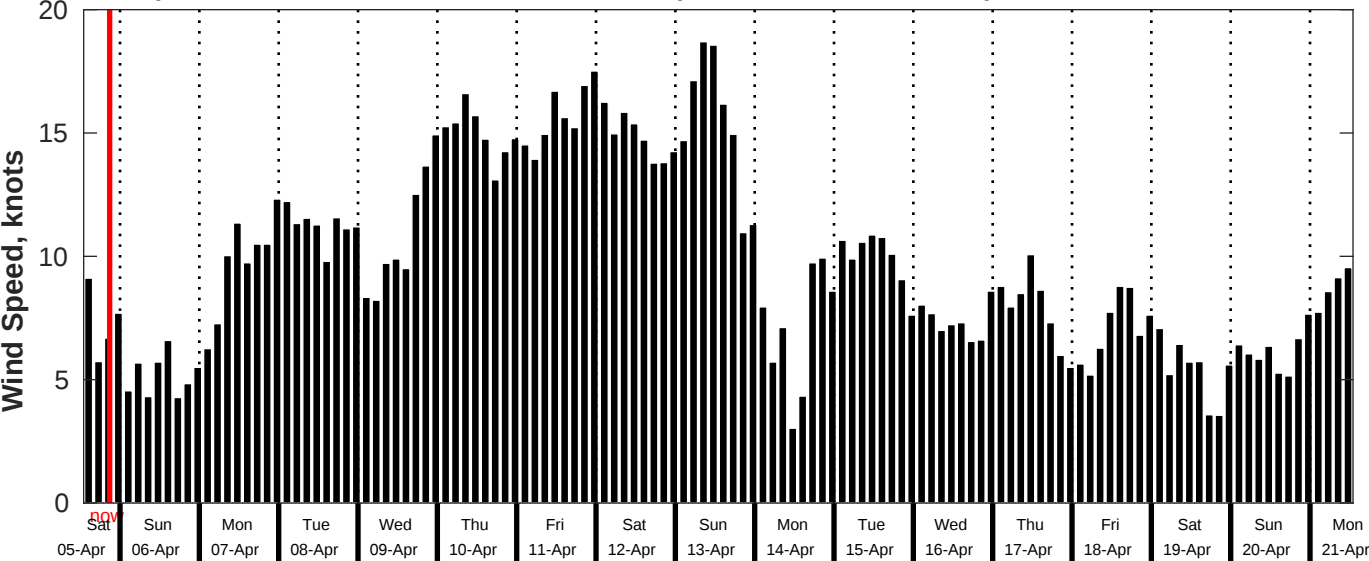
GFS Wind Speed Forecast for NDBC 51209 from 05-Apr-2025 13:00:00 to 21-Apr-2025 13:00:00
