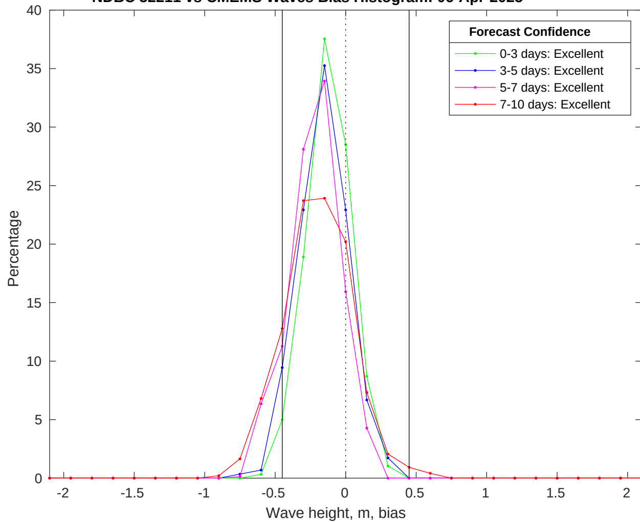
NDBC 52211 vs CMEMS Waves Bias Histogram: 06-Apr-2025
