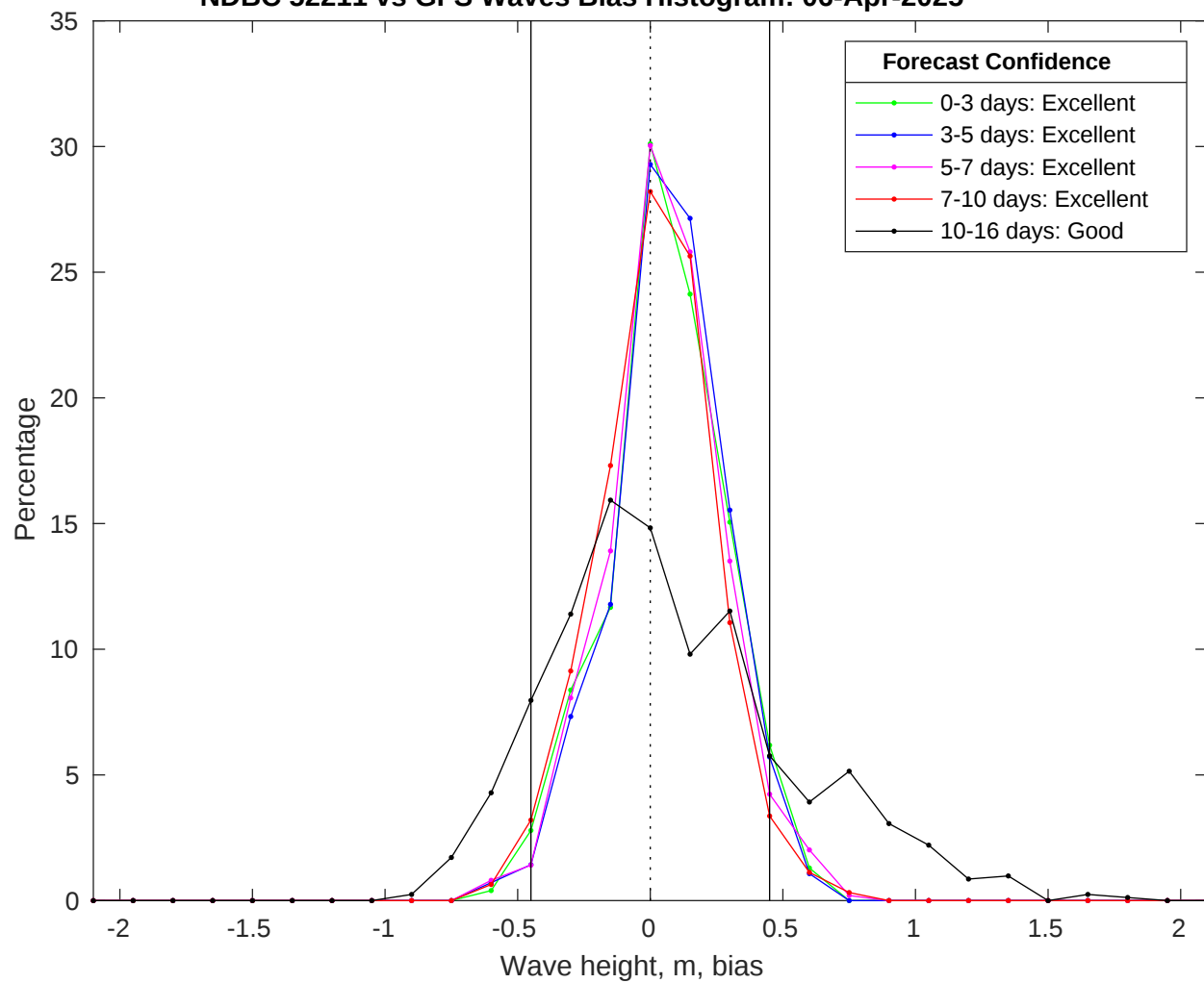
NDBC 52211 vs GFS Waves Bias Histogram: 06-Apr-2025
