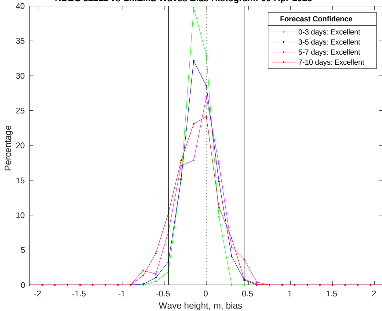
NDBC 52212 vs CMEMS Waves Bias Histogram: 06-Apr-2025
