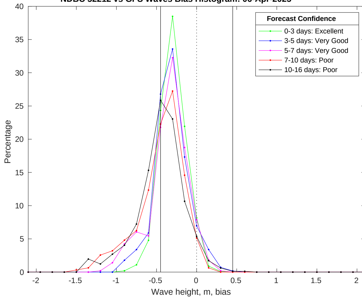
NDBC 52212 vs GFS Waves Bias Histogram: 06-Apr-2025
