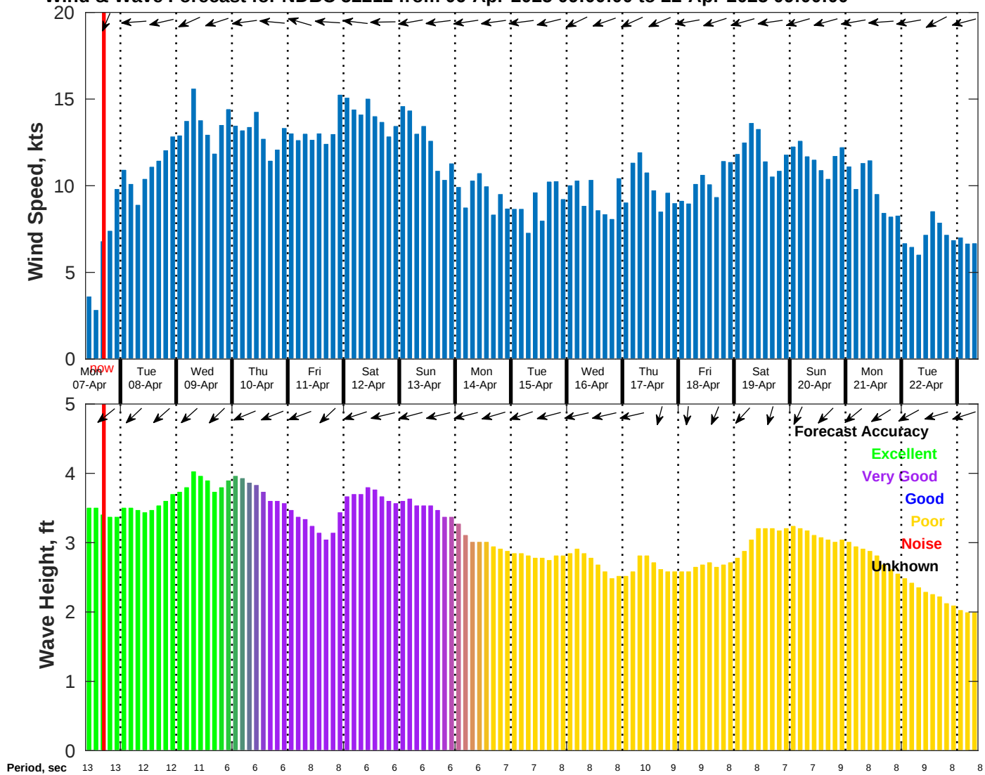
Wind & Wave Forecast for NDBC 52212 from 06-Apr-2025 09:00:00 to 22-Apr-2025 09:00:00
