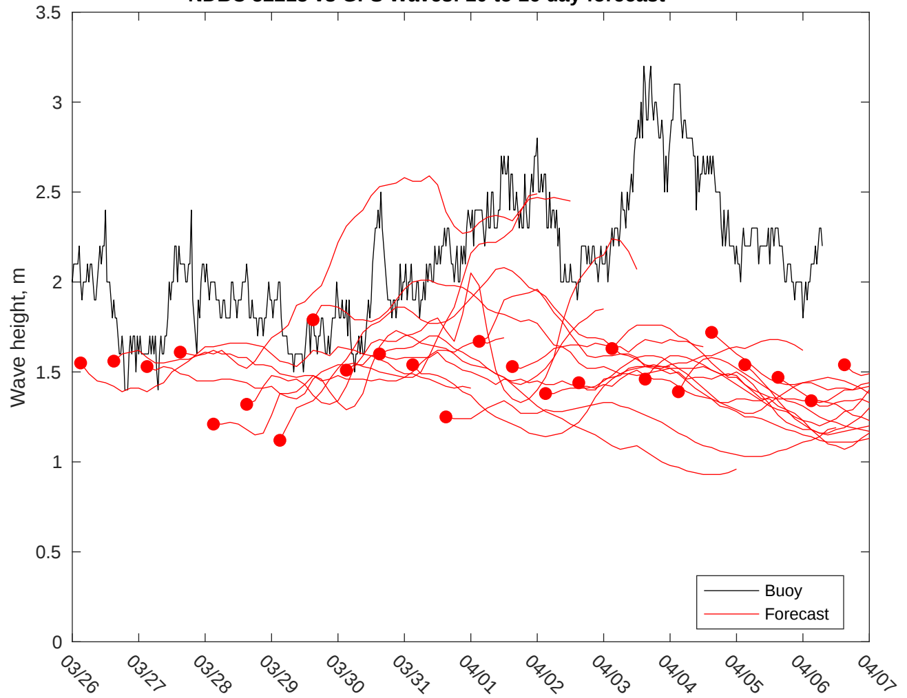
NDBC 52213 vs GFS Waves: 10 to 16 day forecast
