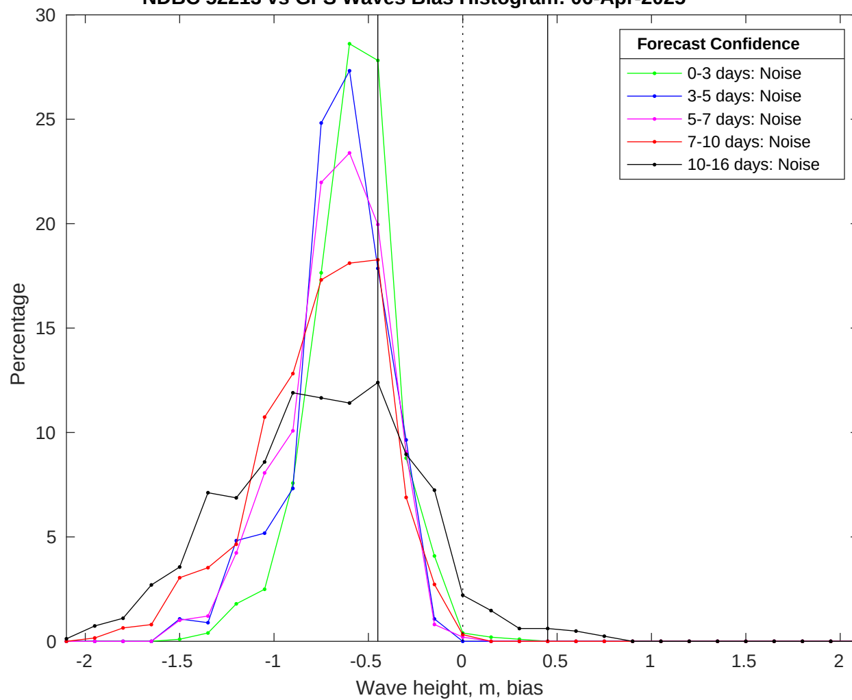
NDBC 52213 vs GFS Waves Bias Histogram: 06-Apr-2025
