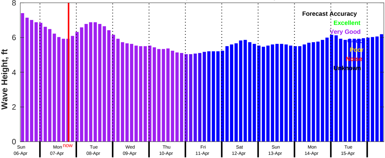
CMEMS Wave Forecast for NDBC 52213 from 05-Apr-2025 11:00:00 to 15-Apr-2025 11:00:00
