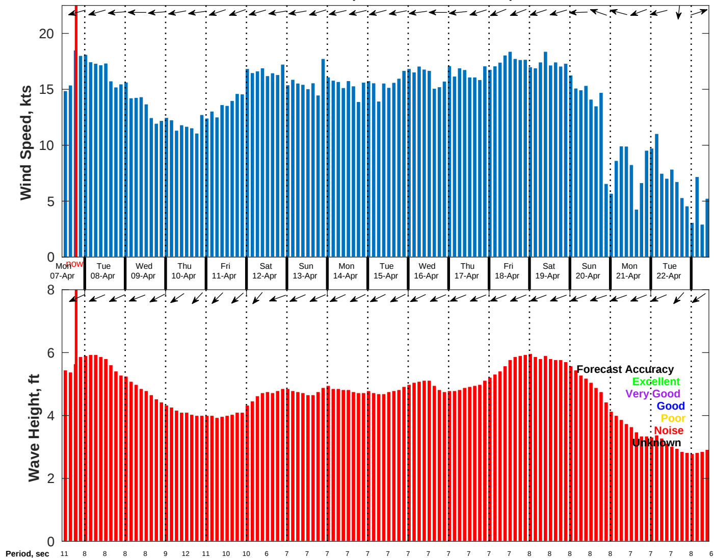
Wind & Wave Forecast for NDBC 52213 from 06-Apr-2025 11:00:00 to 22-Apr-2025 11:00:00
