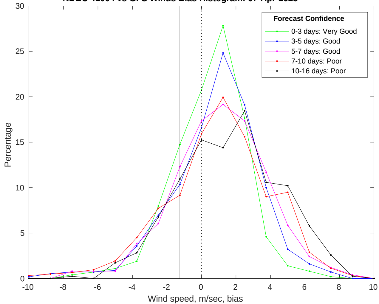
NDBC 41004 vs GFS Winds Bias Histogram: 07-Apr-2025
