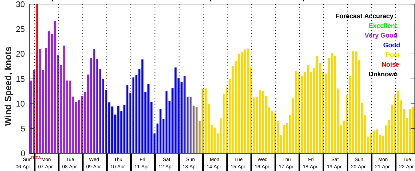
GFS Wind Speed Forecast for NDBC 41004 from 06-Apr-2025 19:00:00 to 22-Apr-2025 19:00:00
