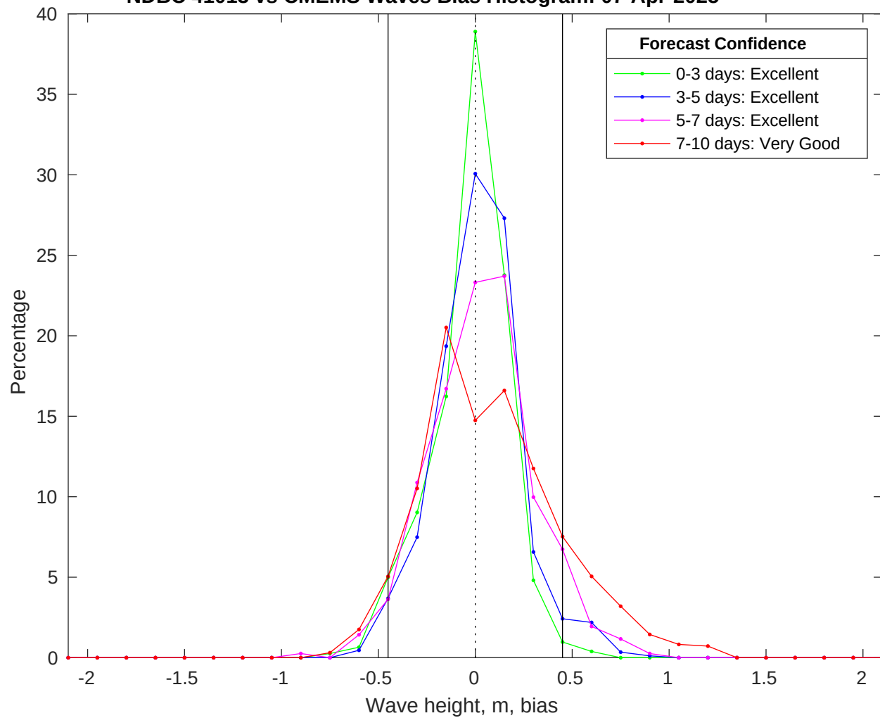
NDBC 41013 vs CMEMS Waves Bias Histogram: 07-Apr-2025
