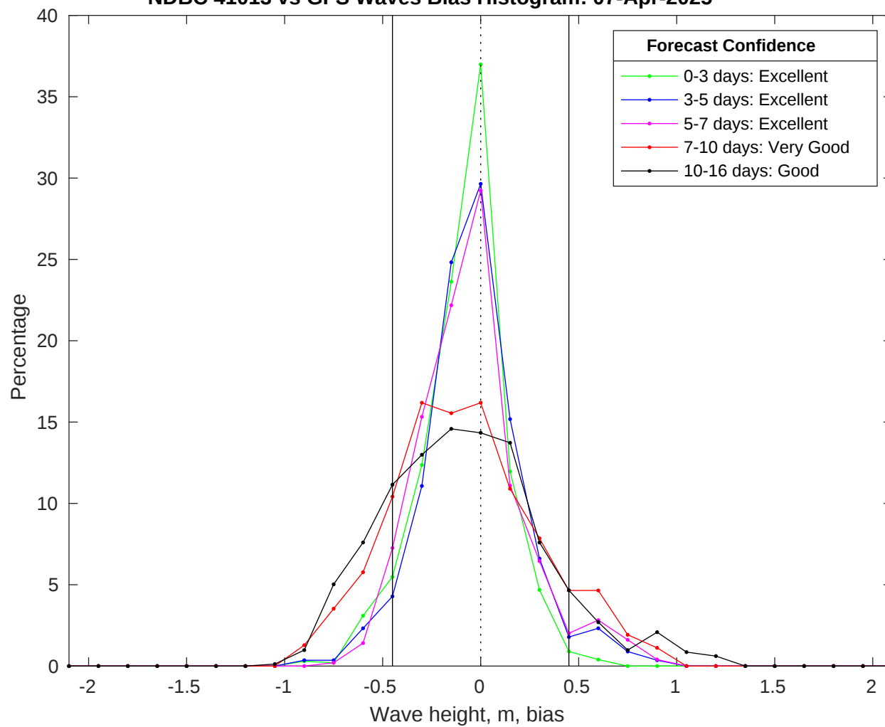
NDBC 41013 vs GFS Waves Bias Histogram: 07-Apr-2025
