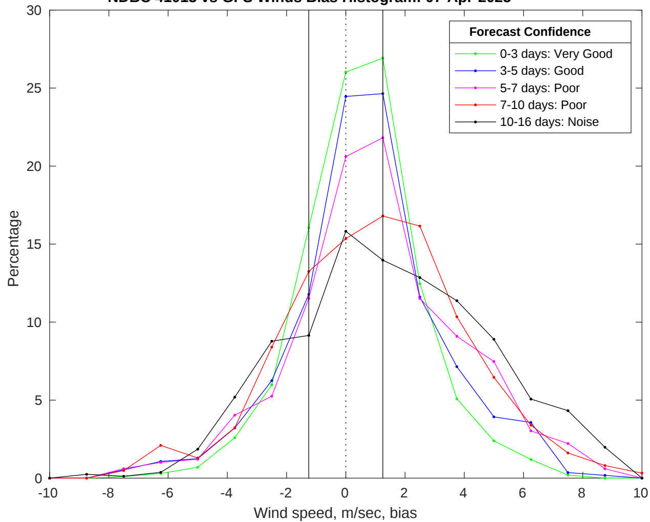
NDBC 41013 vs GFS Winds Bias Histogram: 07-Apr-2025
