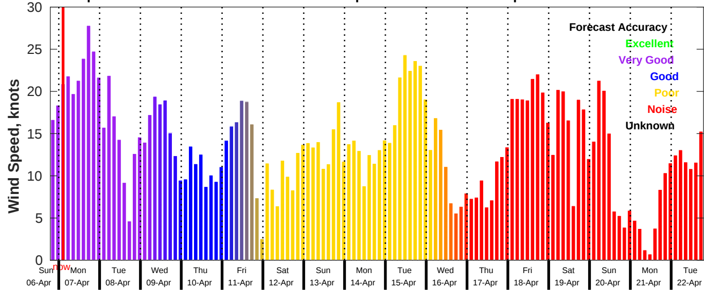
GFS Wind Speed Forecast for NDBC 41013 from 06-Apr-2025 19:00:00 to 22-Apr-2025 19:00:00
