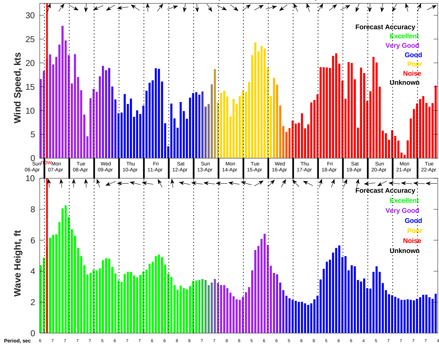
Wind & Wave Forecast for NDBC 41013 from 06-Apr-2025 19:00:00 to 22-Apr-2025 19:00:00
