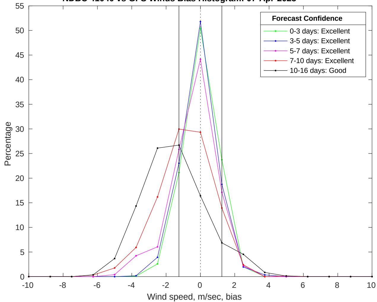
NDBC 41040 vs GFS Winds Bias Histogram: 07-Apr-2025
