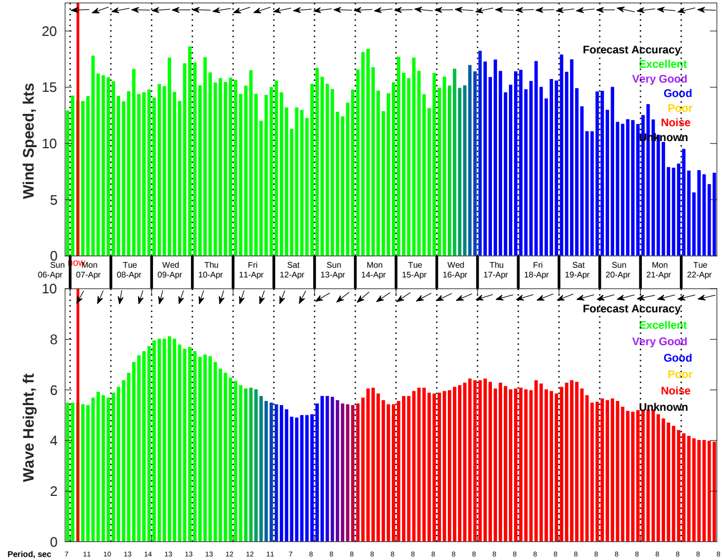
Wind & Wave Forecast for NDBC 41040 from 06-Apr-2025 21:00:00 to 22-Apr-2025 21:00:00
